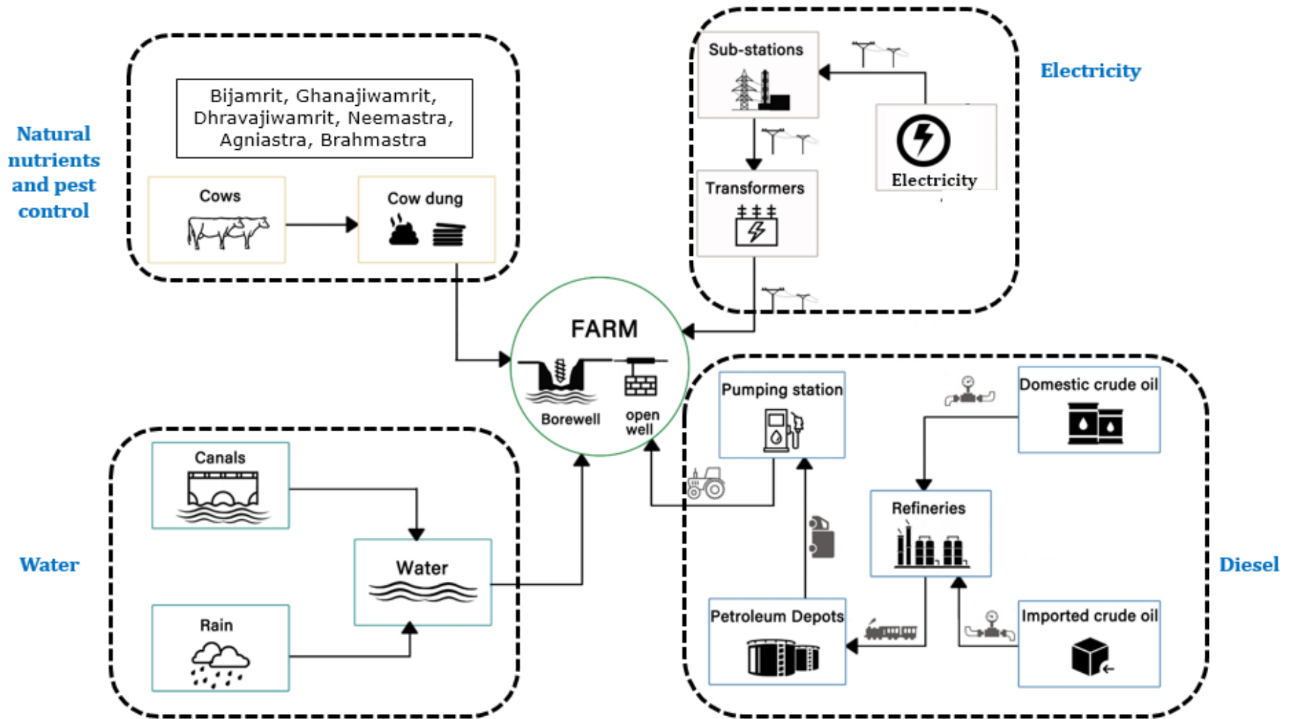
Figure 2.2: Methodology to assess the life cycle energy and emissions for ZBNF
